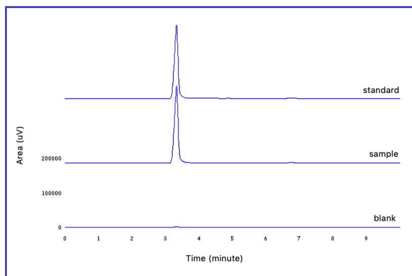
Figure 3. HPLC chromatogram of glucosamine hydrochloride (C18 Lichrospher® 100 endcapped, 250 \times 4.0 mm i.d., 5\text{ }\mu\text{m} ; mobile phase: 0.5 g sodium pentane sulfonate dissolved in 800 mL water + 4 mL 1M potassium hydroxide, diluted to 1000 mL with water, 430\text{ }\mu\text{L} perchloric acid, and 50 mL acetonitrile; flow rate: 0.5 mL/min; detection: 195 nm with DAD).
